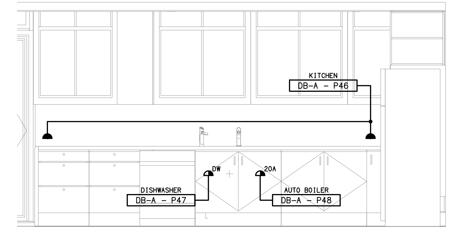
DETAIL A KITCHENETTE ELEVATION 1 SCALE 1:25
