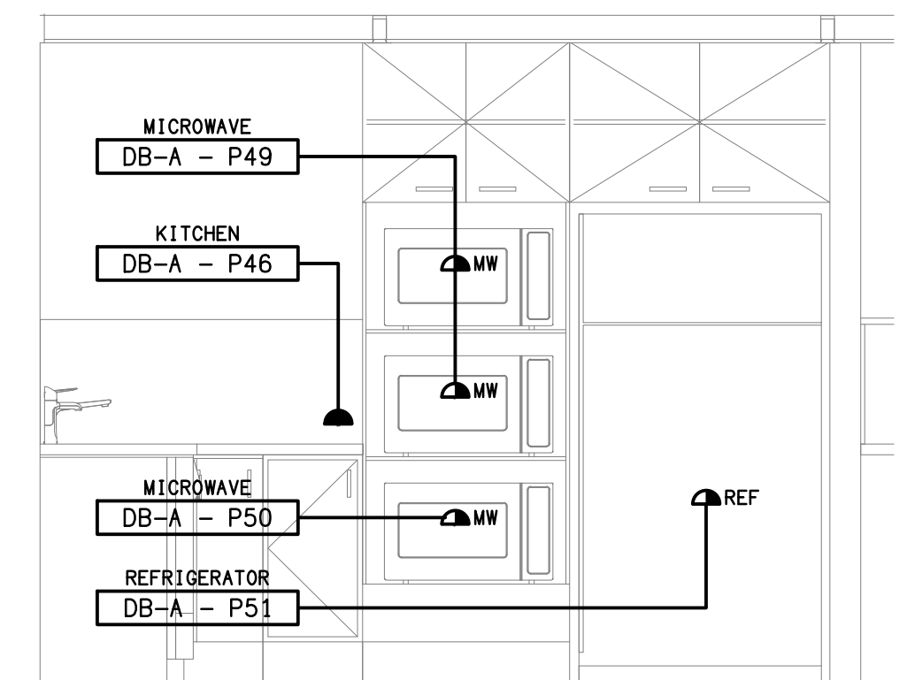
DETAIL B KITCHENETTE ELEVATION 2 SCALE 1:25
