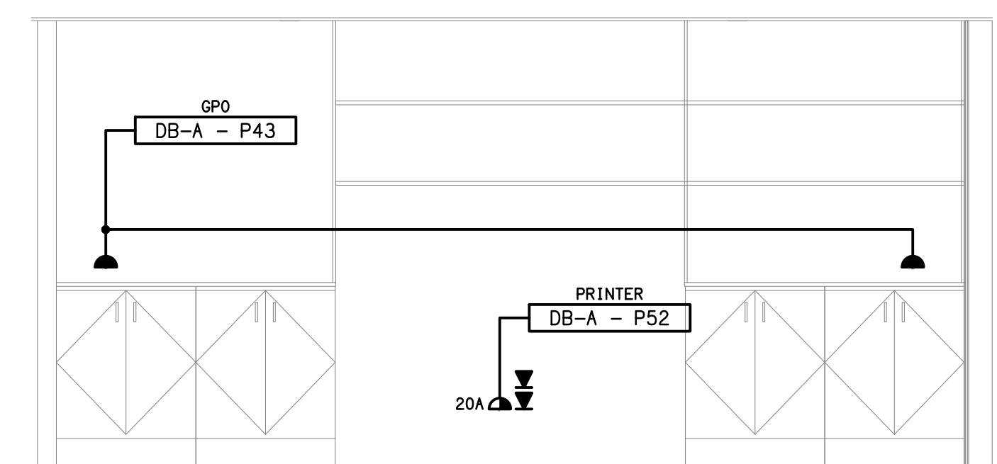
DETAIL C UTILITY BENCHES ELEVATION SCALE 1:25
